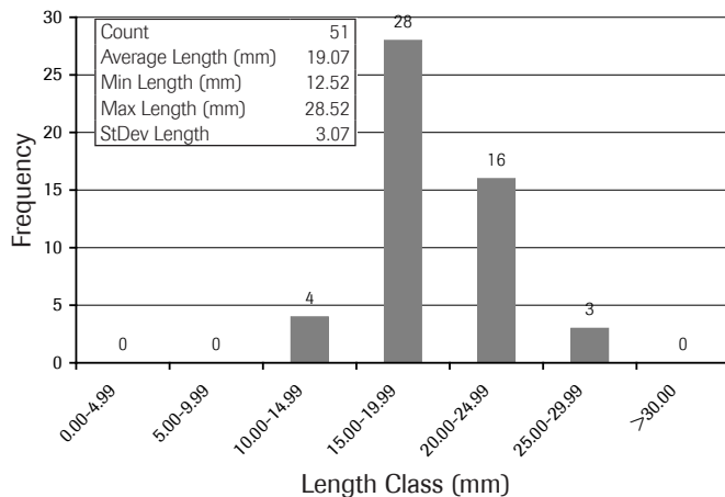
Figure 4. Length-frequency analysis for 51 zebra mussels collected in the Housatonic River (October 2009).
